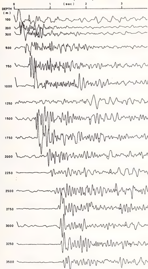
Fig. 5 Records of the horizontal component seismometer with the suitable filtering. Solid circles show the detected onset of S wave.
